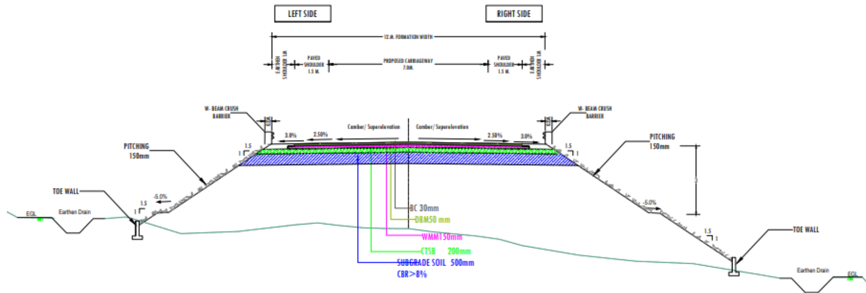
Fig. 2.9 Modified As per IRC SP 73: 2018
